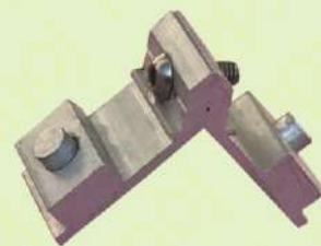
MH-1242 SECTION FLAT
